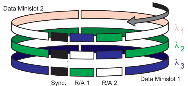
Fig. 5. The slots on the data channels may be thought of as ribbons with the locations of minislots marked on them. The slots on each channel are synchronized. The shade of each R/A minislot shows which node this minislot is allocated to — note that these cyclically permute so that a node only needs to place requests and allocations onto one channel at a time.
