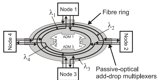
Fig. 1. Four-node MAWSON ring.
